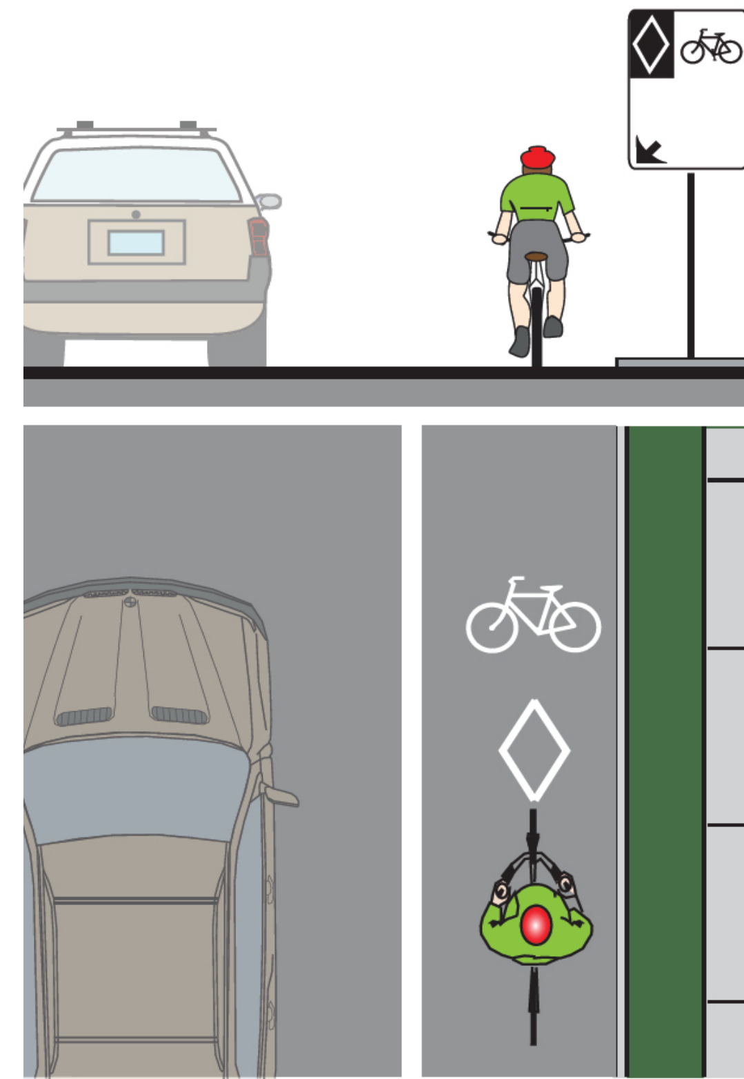
CONVENTIONAL BIKE LANE
