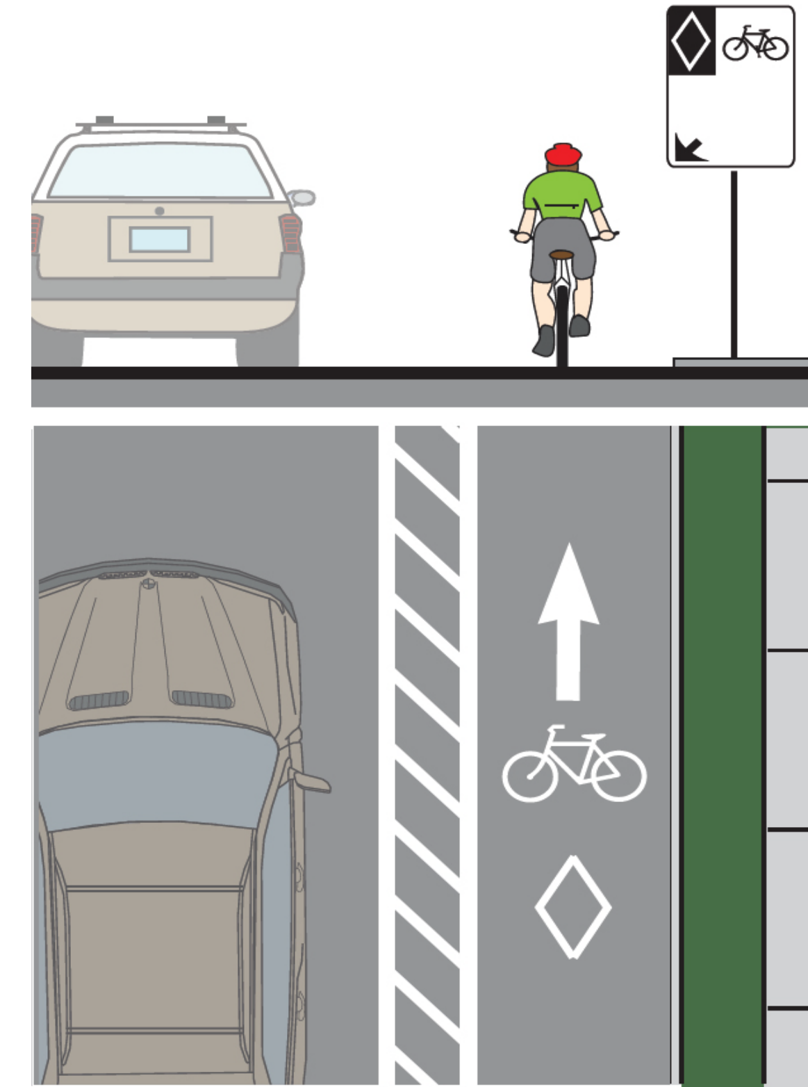
BUFFERED BIKE LANE
